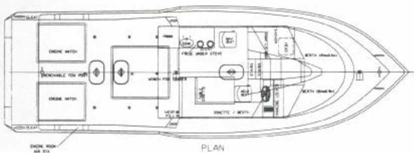
PLAN
