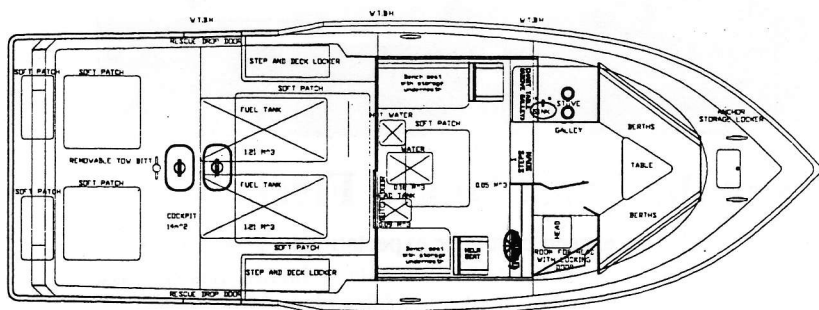
MetalCraft Marine designed Canadian Coast Guard 40' RER/SAR Cutter
